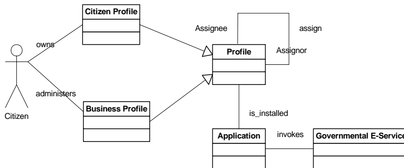
Figure 1: OpenSocialGov Interaction Model
